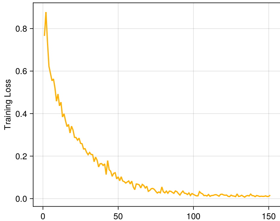
Outer Fold 4
