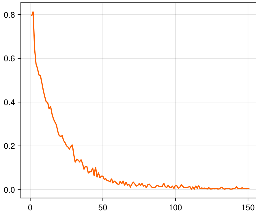
Outer Fold 5
