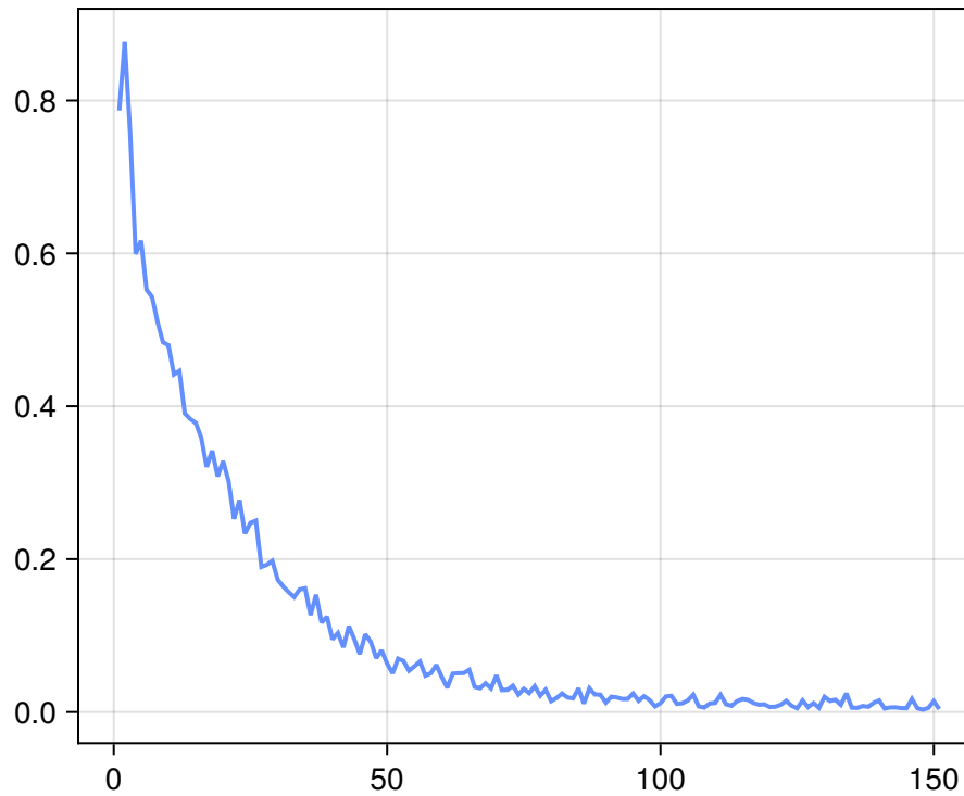
Outer Fold 5
